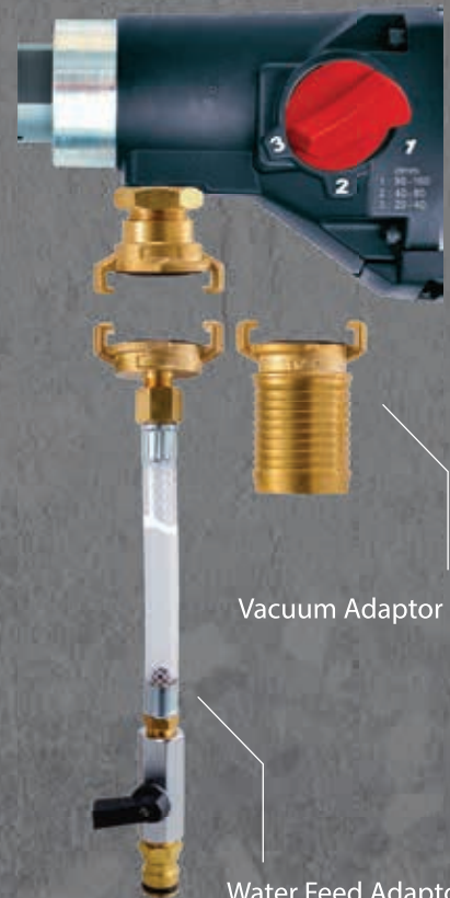
Water Feed Adaptor Head
